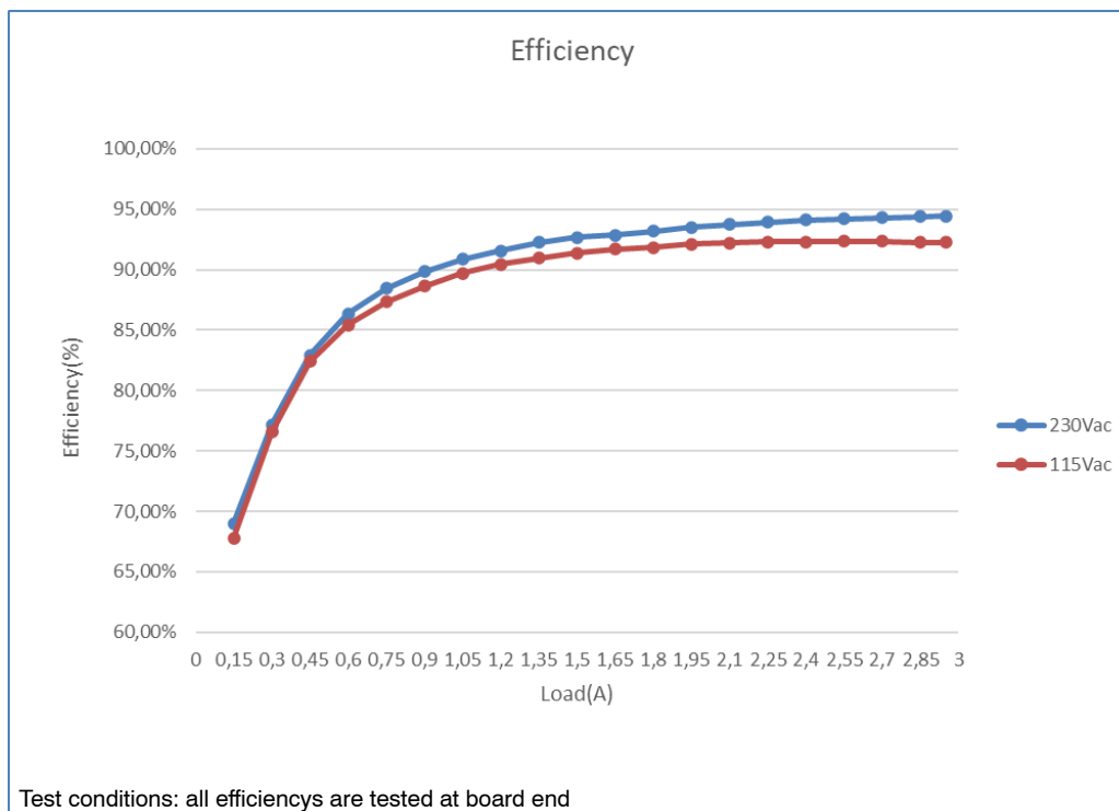
Figure 16. Efficiency Curve
