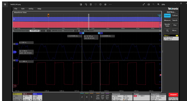
Figure 23. 50 V/3 A
