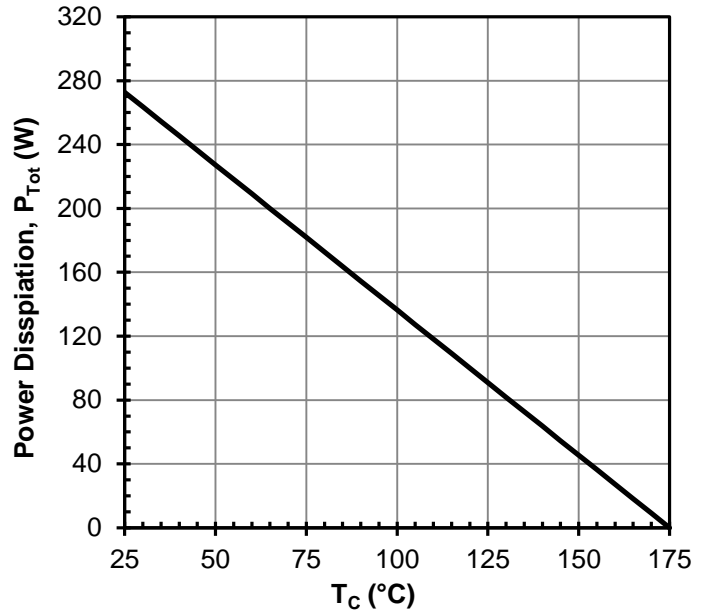
Figure 4 Power dissipation
