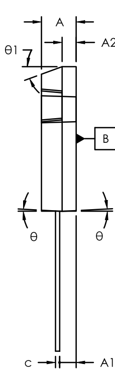
TO247-3 15.90x20.96x5.03, 5.44P CASE 340AK ISSUE A
