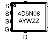
DFN5 (SO-8FL) CASE 488AA
