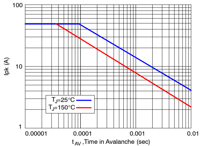
Figure 12. I_{pk} vs. Time in Avalanche (UIS)
