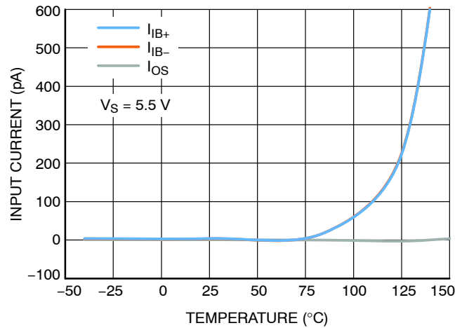
Figure 11. Input Current vs. Temperature
